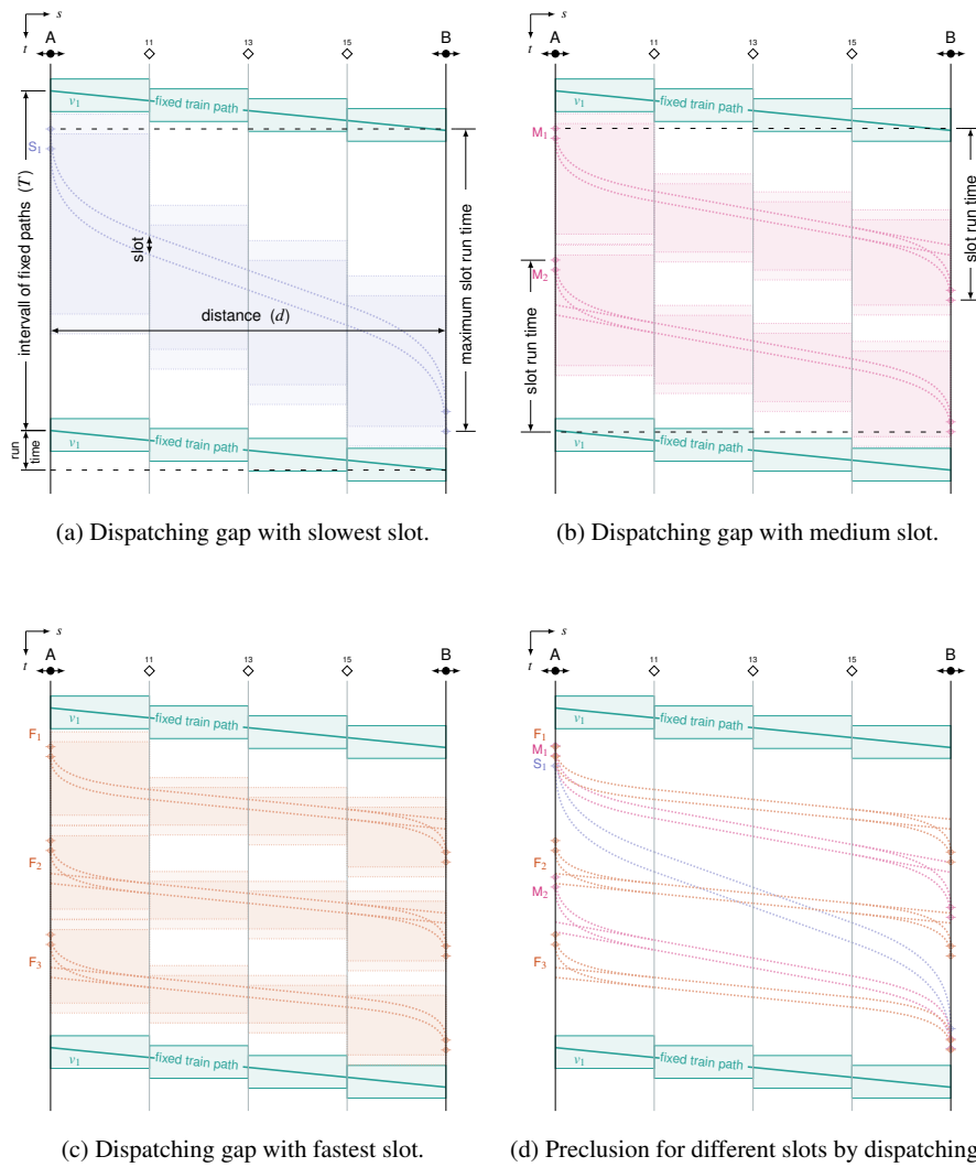
Figure 7: Utilisation of dispatching gap with slots.
