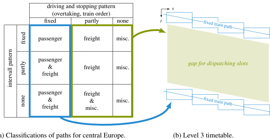
Figure 6: Paths classifications and their accommodation in a Level 3 timetable.
